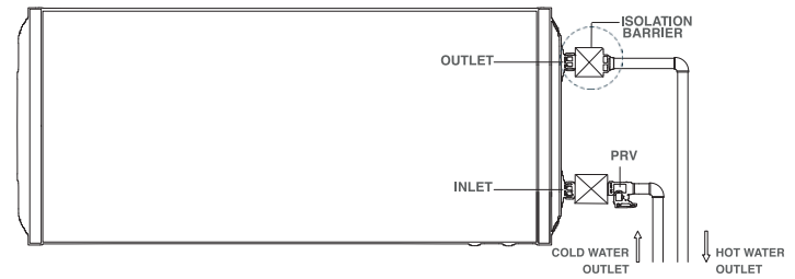
Pipe Connection
