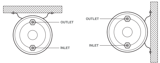
Ceiling Mounting
