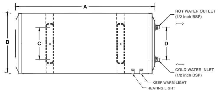
Product Structure
